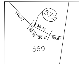
DETAIL SCALE 1" = 50'
