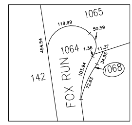
DETAIL SCALE 1" = 100'
