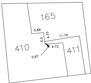
DETAIL SCALE - 1" = 10'
