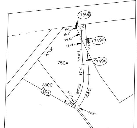
DETAIL SCALE 1" = 200'
